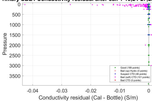
Primary SBE4 Conductivity residual after cal. 1-19,24-27,29,31,33
