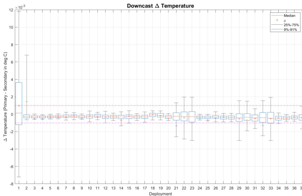
Figure 3: Difference (primary - secondary) between temperature sensor values on downcast
