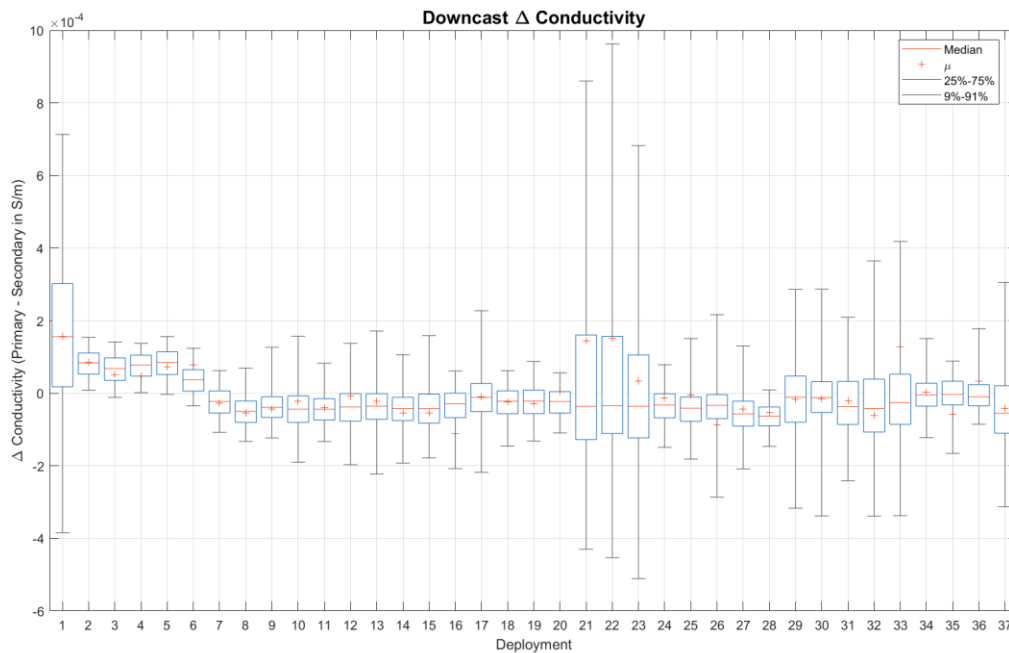
Figure 5: Difference (primary - secondary) between conductivity sensor values on downcast
