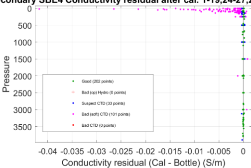
Secondary SBE4 Conductivity residual after cal. 1-19,24-27,29,31,33
