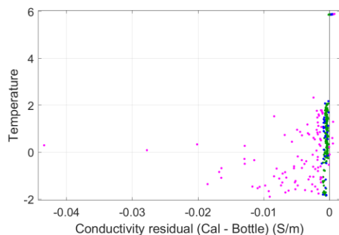
Secondary SBE4 Conductivity residual before cal. 1-19,24-27,29,31,33
