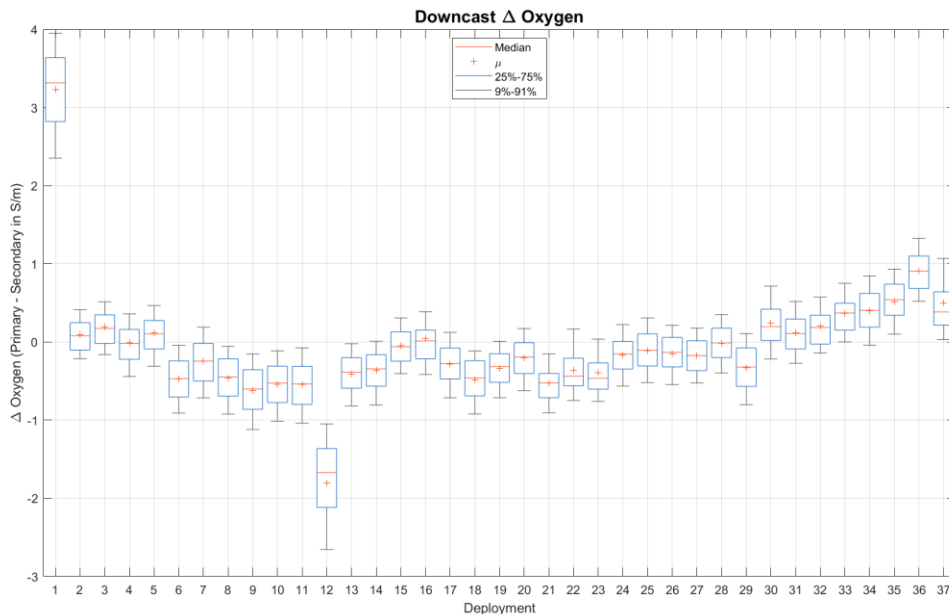
Figure 7: Difference (primary - secondary) between dissolved oxygen sensor values on downcast
