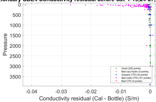
Secondary SBE4 Conductivity residual before cal. 1-19,24-27,29,31,33
