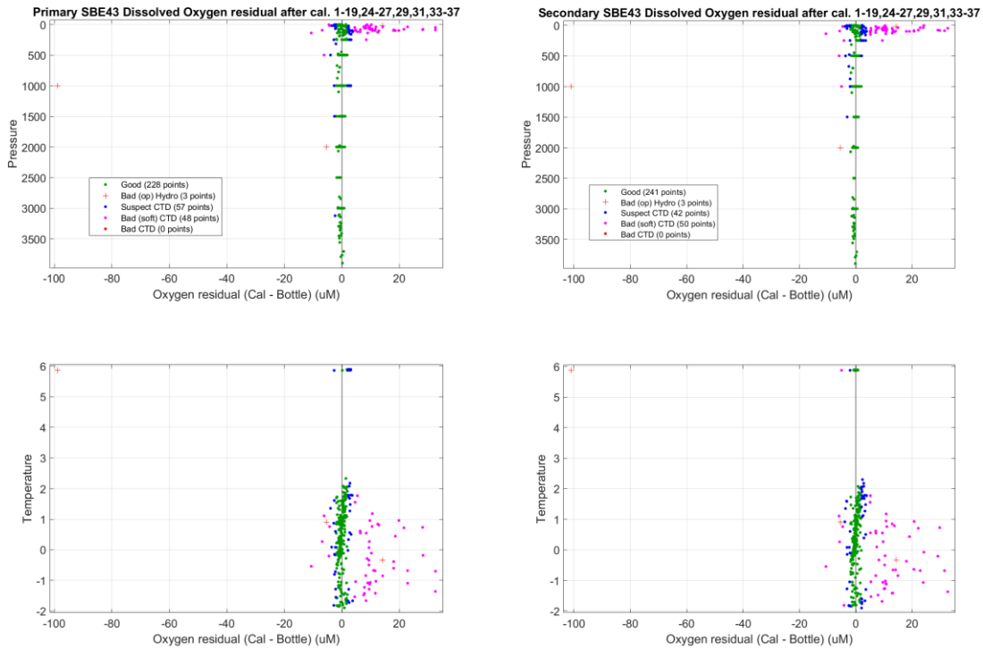
Figure 6: CTD SBE43 - bottle dissolved oxygen difference and calibration error (left: primary, right: secondary)
