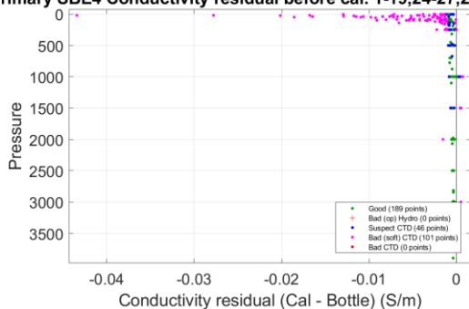
Primary SBE4 Conductivity residual before cal. 1-19,24-27,29,31,33
