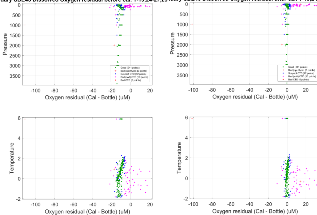
Primary SBE43 Dissolved Oxygen residual before cal. 1-19,24-27,29,31,33 Primary SBE43 Dissolved Oxygen residual after cal. 1-19,24-27,29,31,33
