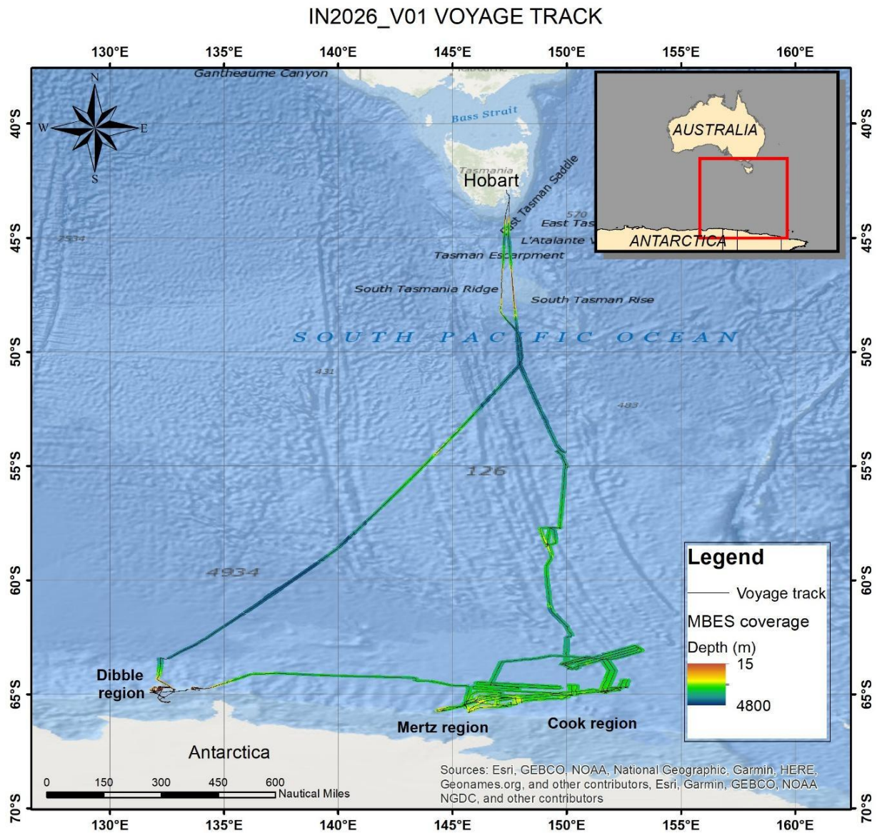
Figure 1: Voyage track
