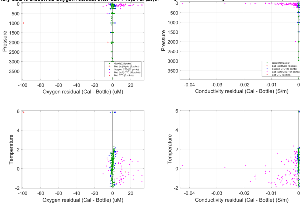
Primary SBE43 Dissolved Oxygen residual after cal. 1-19,24-27,29,31,33 Primary SBE4 Conductivity residual after cal. 1-19,24-27,29,31,33
