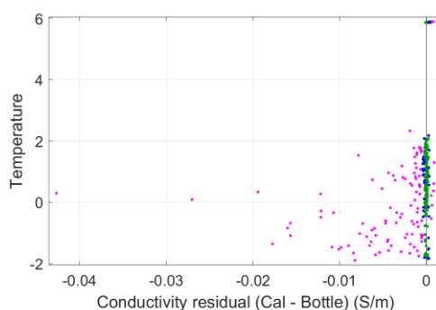
Secondary SBE4 Conductivity residual after cal. 1-19,24-27,29,31,33
