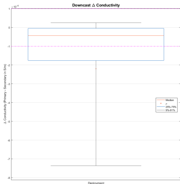
Figure 6: Difference (primary - secondary) between conductivity sensor values on downcast
