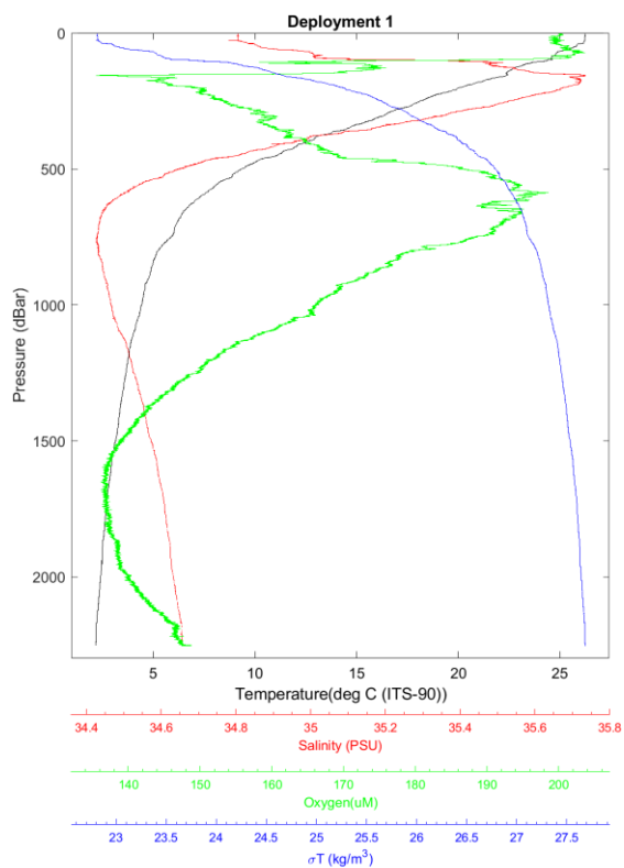
Figure 5: Temperature, salinity, dissolved oxygen and \sigma_T profiles
