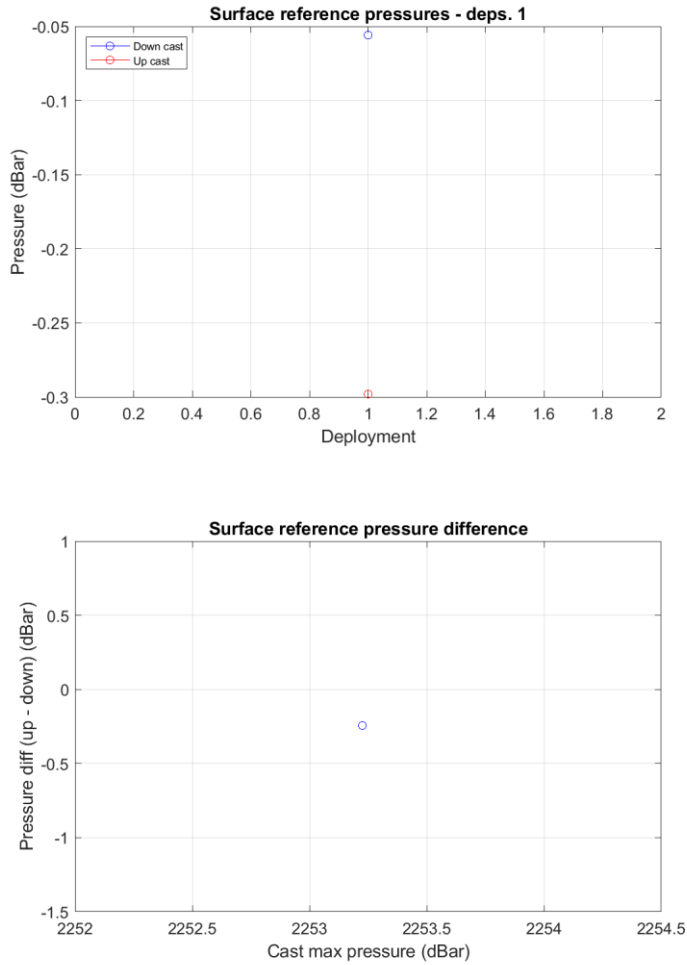
Figure 2: CTD pressure offsets
