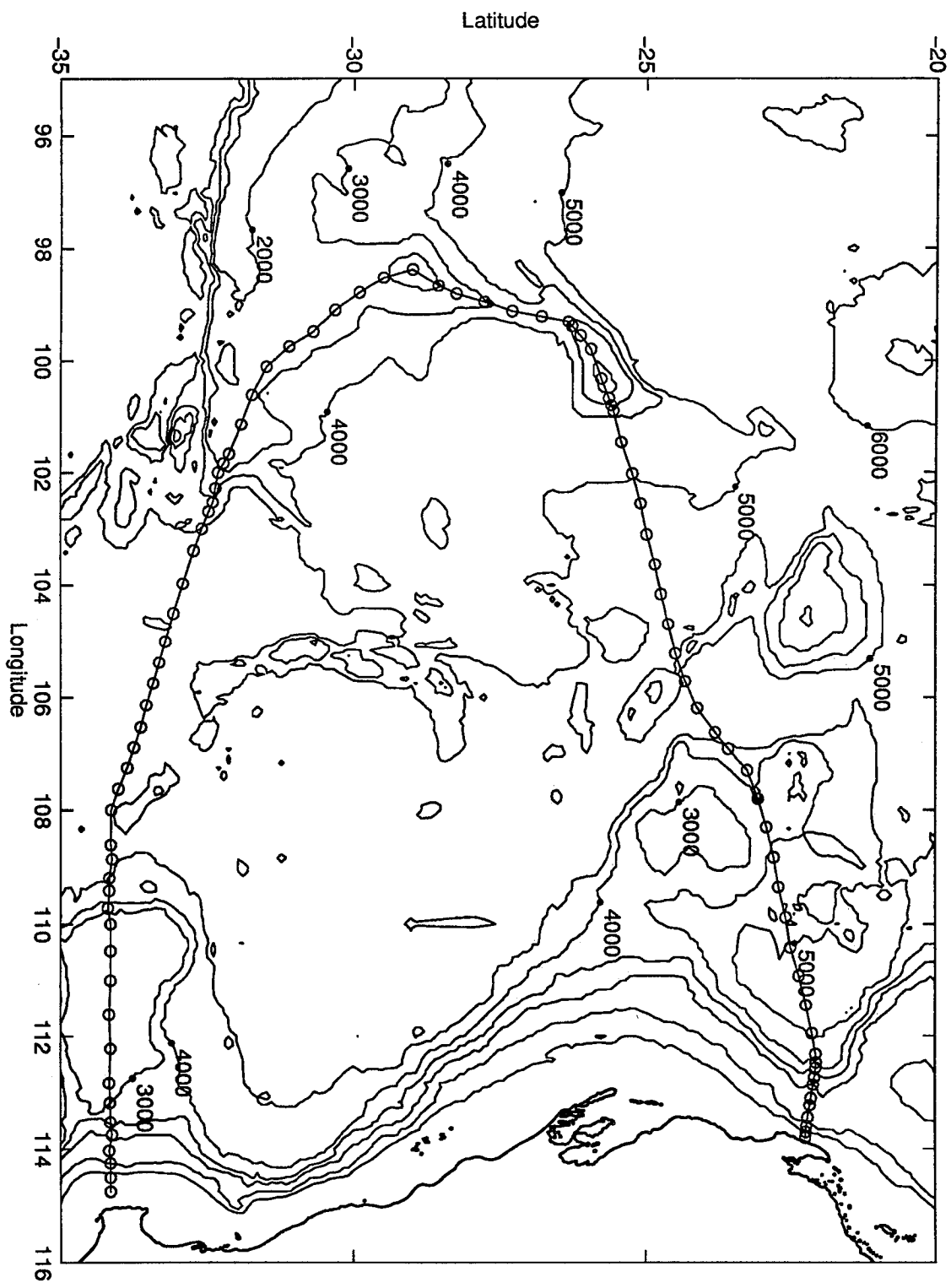
Figure 1: FR 05/96 Actual Cruise Track and location of CTD's.
