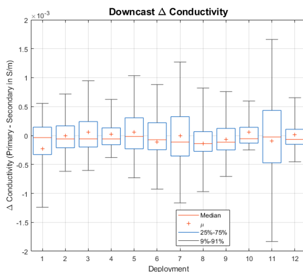
Figure 5 Difference between primary and secondary conductivity sensors
