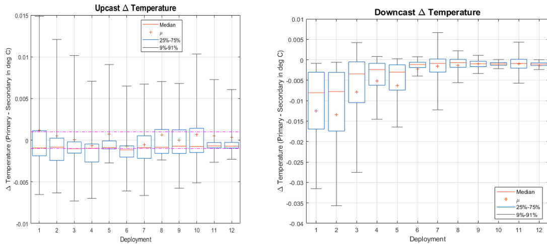
Figure 3 Difference between primary and secondary temperature sensors
