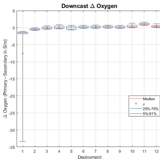
Figure 7 Difference between primary and secondary Dissolved Oxygen sensors
