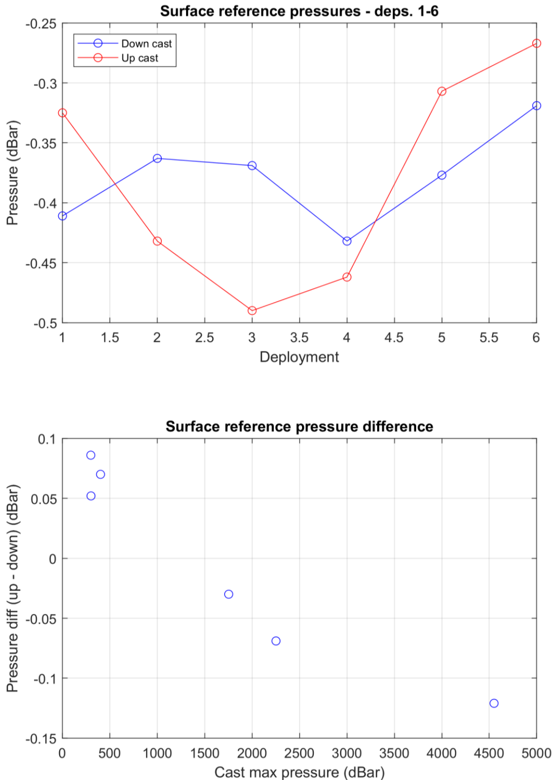
Figure 2 CTD pressure offsets
