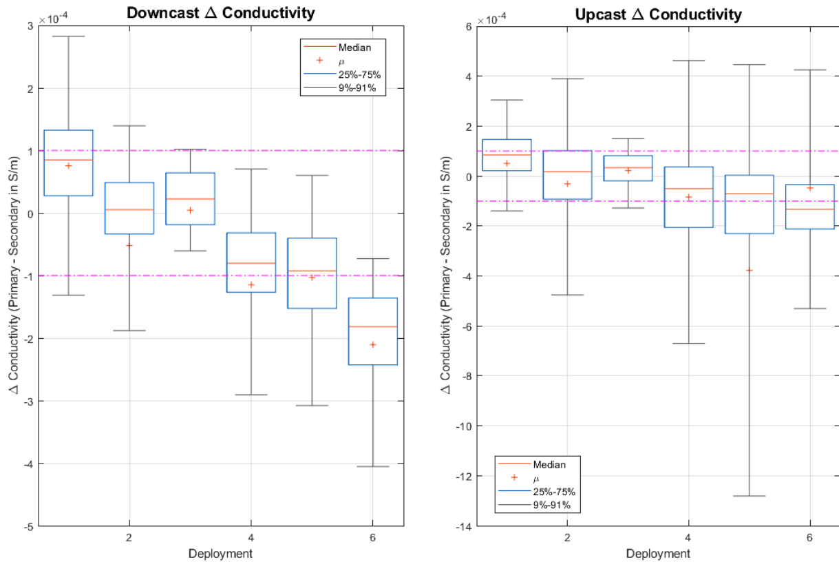
Figure 5 Difference between primary and secondary conductivity sensors
