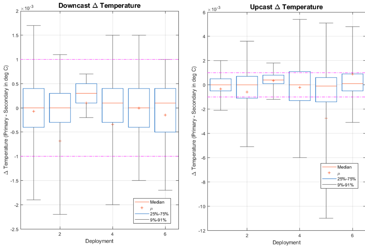
Figure 3 Difference between primary and secondary temperature sensors
