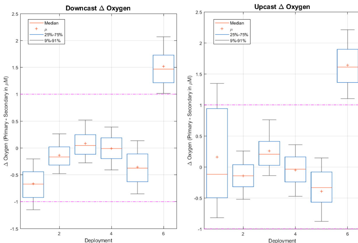
Figure 7 Difference between primary and secondary Dissolved Oxygen sensors
