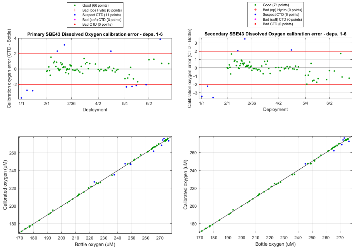
Figure 6 Dissolved Oxygen Difference with upcast CTD data (SBE43 - Bottle)
