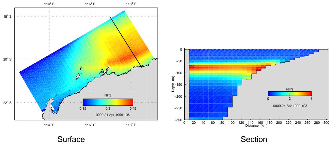
Figure 4.1.9: Ammonia distribution ( \text{mg N m}^{-3} ).
