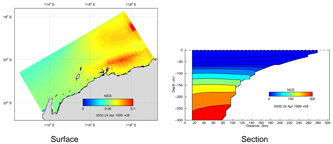
Figure 4.1.8: \text{NO}_3 distribution ( \text{mg N m}^{-3} ) Contours in the section are 0.01, 0.1, 1, 10, 25, 50, 100, 150, 200, 250.
