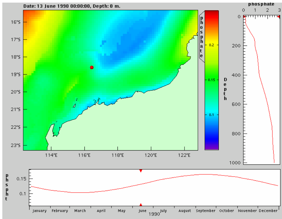
Figure 3.1.4: \text{PO}_4 distribution from CARS (micromolar).
