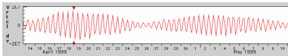
Figure 4.3.13 (a): Sample maximum instantaneous vertical advective flux through 80 m depth. This time series was taken at 250 m depth on the Port Hedland section.
