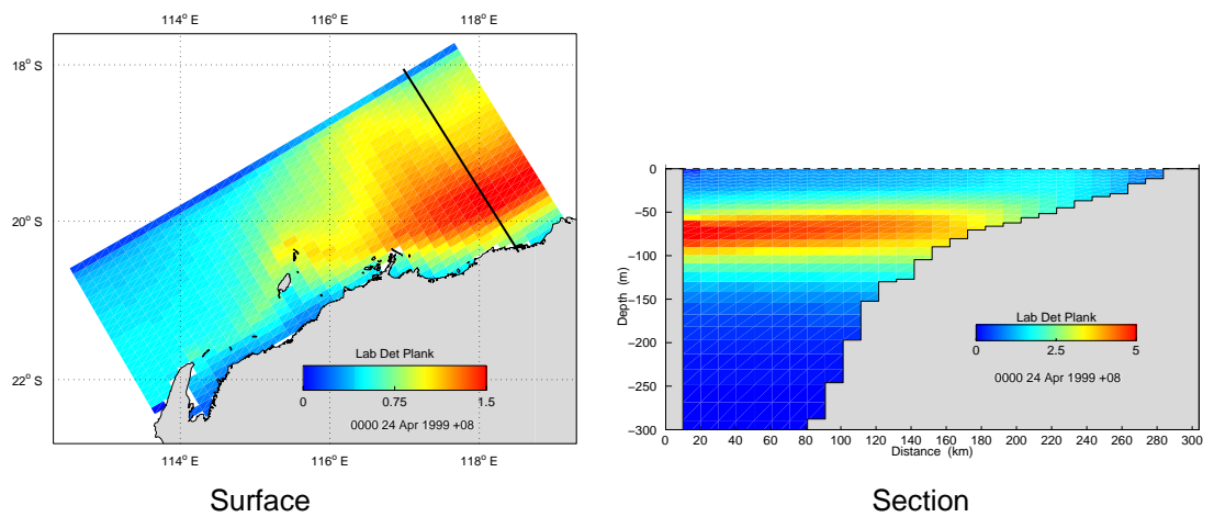
Figure 4.1.10: Planktonic labile detrital Nitrogen distribution ( \text{mg N m}^{-3} ).
