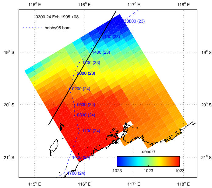
Figure 4.7.3 (a): Section orientation and cyclone passage for density sections. Note: 1800 hours corresponds to the cyclone centre approximately midway along the section.
