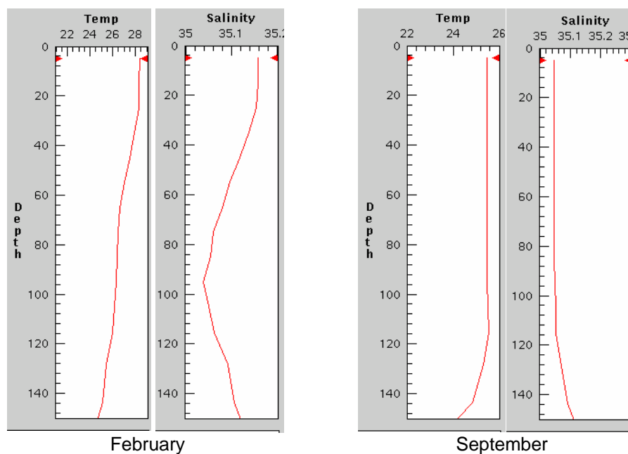
Figure 4.5.11: Temperature ( ^{\circ}\text{C} ) and salinity (psu) output from ACOM3.
