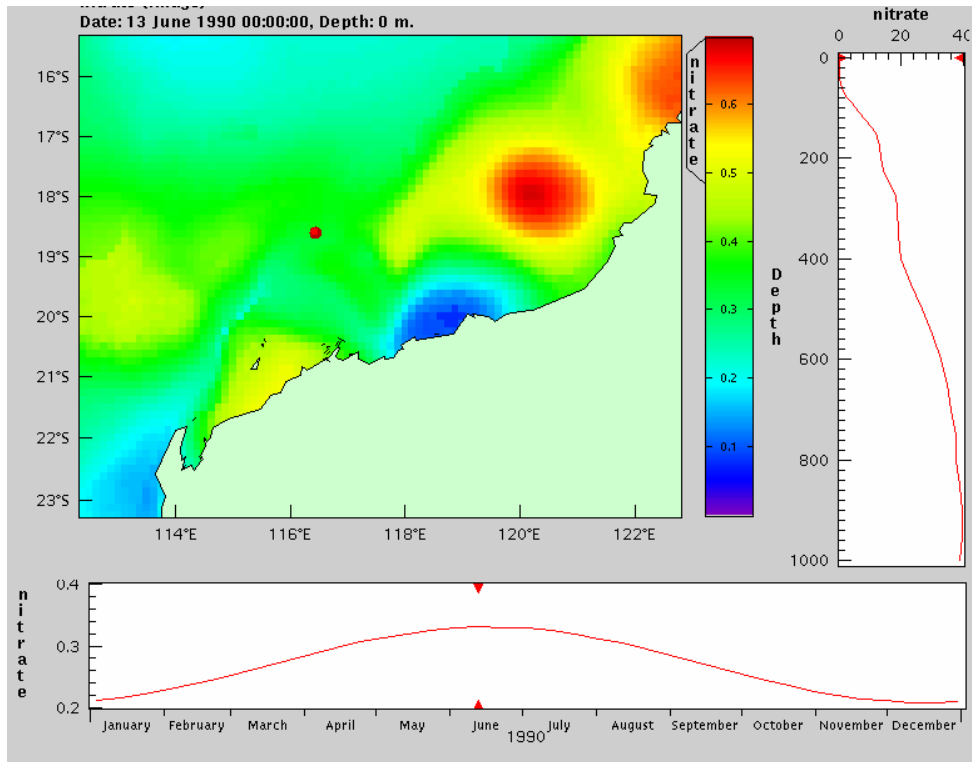
Figure 3.1.3: \text{NO}_3 distribution from CARS (micromolar). Depth profile and (surface) annual time series are taken at the location of the red dot.
