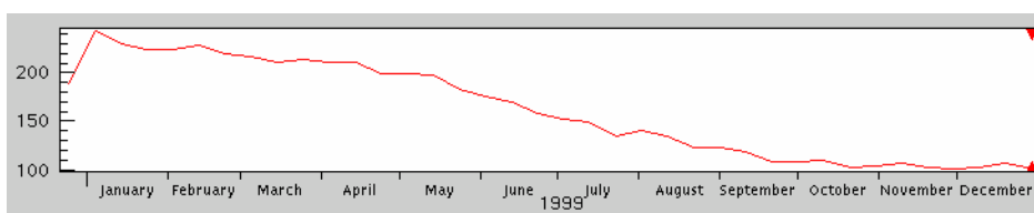
Figure 4.3.5: Nitrate time series at mid-domain, 200 m depth ( \text{mg N m}^{-3} ).
