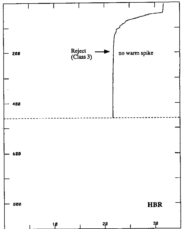
Figure 3.1R Hit Bottom Reject (HBR)
