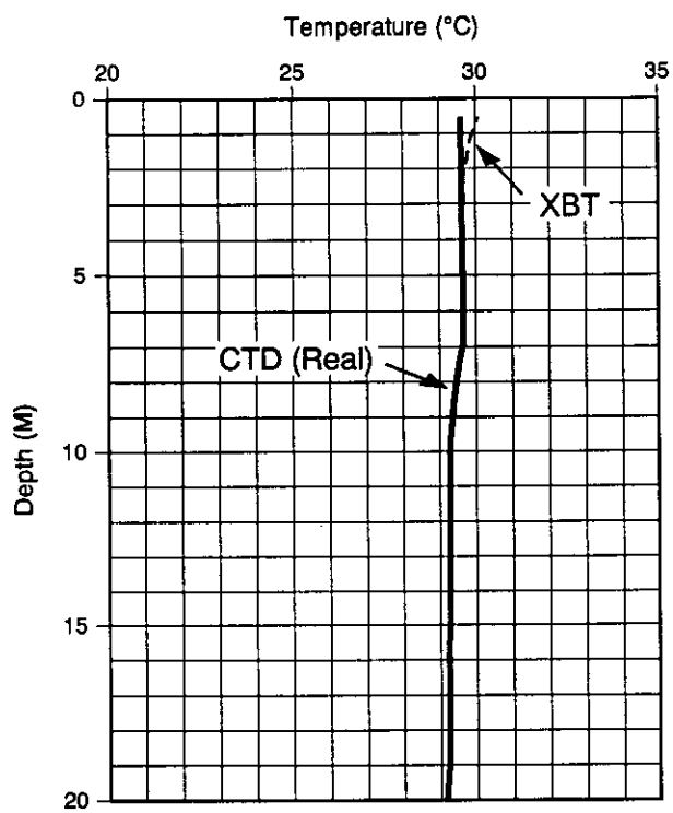
Figure 2.1 Surface Spike Start up Transient Problem (CS)
