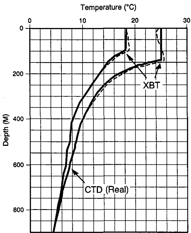
Figure 2.6 Bathy Systems Bowing Problem or Bowed Mixed Layer
