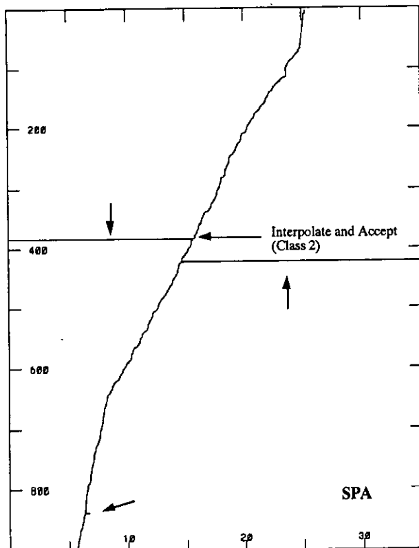
Figure 3.3A Spikes Accept (SPA)
