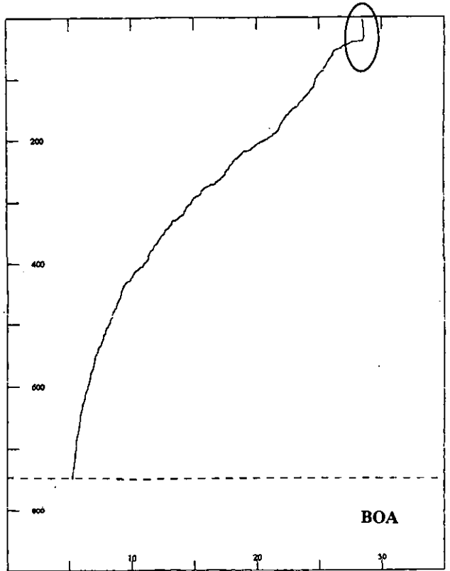
Figure 2.6A Bowed Mixed Layer Accept (BOA)
