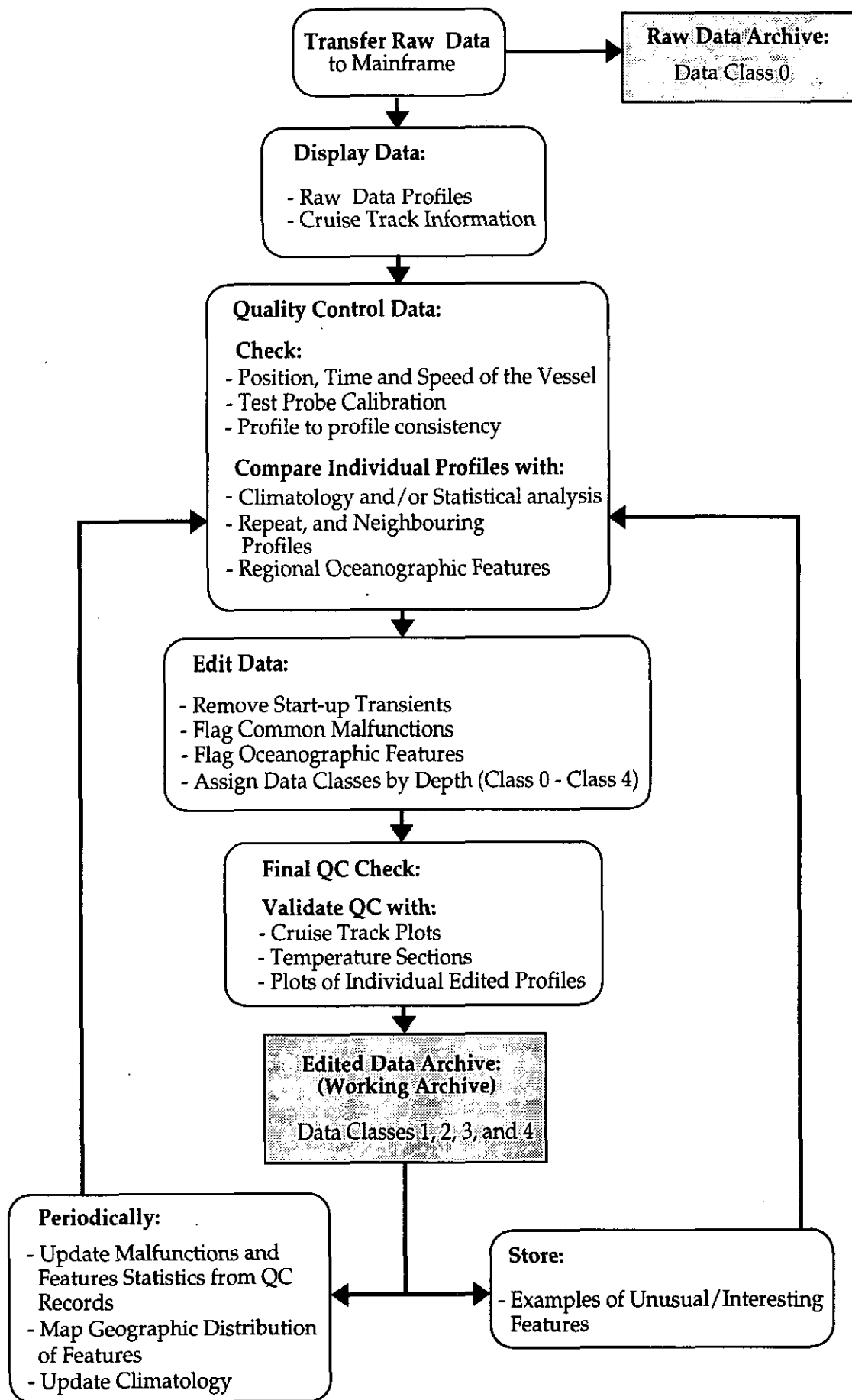
Figure 2 CSIRO XBT Quality Control Process
